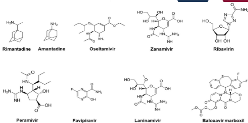
Figure 1: Typical antiviral drugs used to treat influenza and their molecular structures
